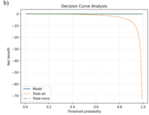
Figure 1. Held-out ROC (a) and decision-curve analysis (b) for the exported corrected forward model. The model retained good ranking performance over a good threshold range.
